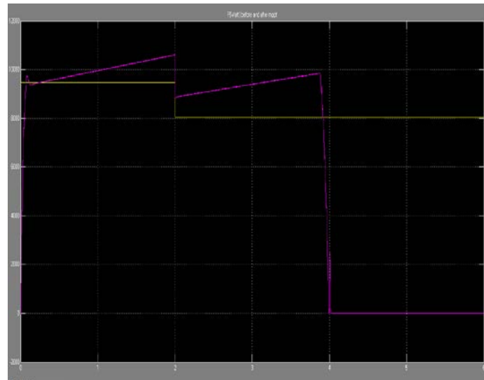
Fig. 6: Tracking of MPP in Power curve of solar module after MPPT
