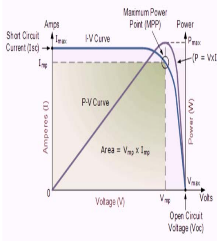
Fig.3: Combined I-V and P-V Curve of PV Module
