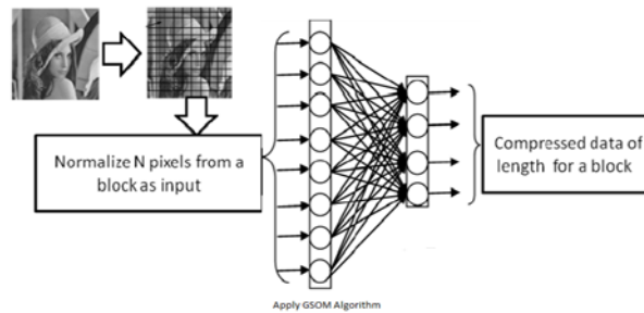
Figure 1: GSOM Architecture compression
