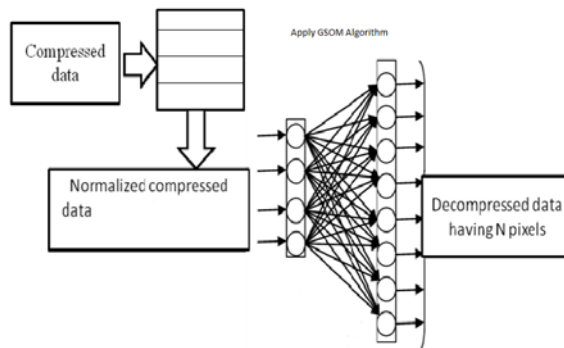
Figure 2: GSOM Architecture decompression
